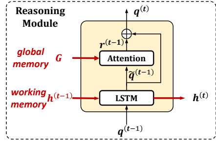
Figure 2: The detailed structure of reasoning module.
